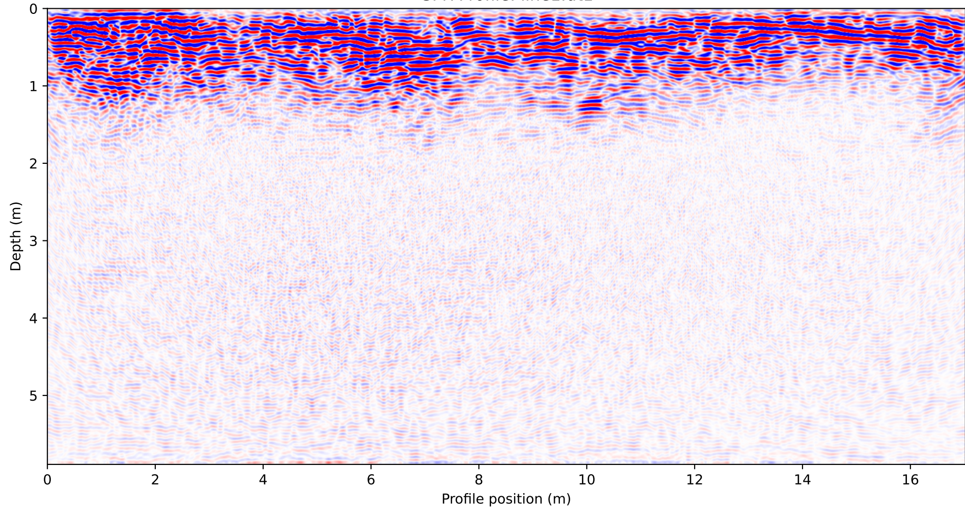
GPR Profile: line1.dt1
